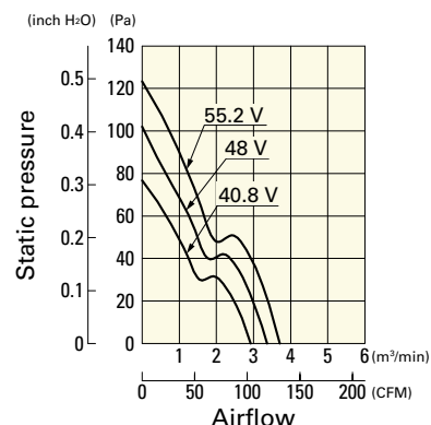
9G1248M101 With pulse sensor
